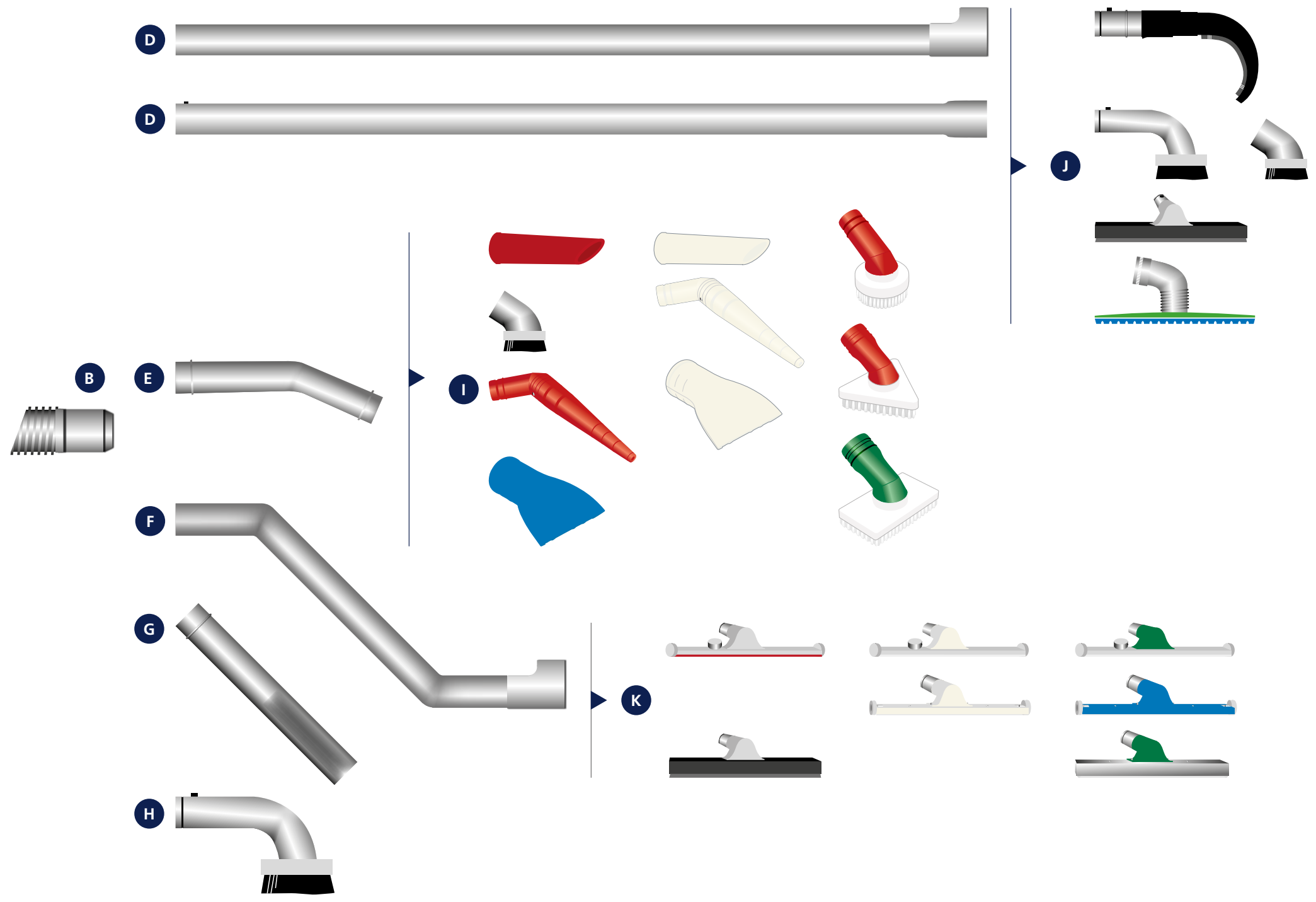
CONNECTION DIAGRAMS
